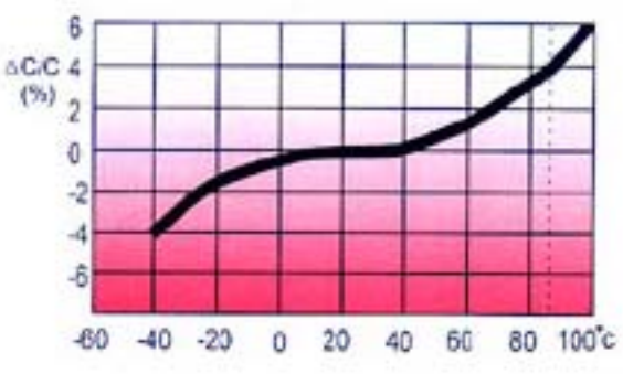
Capacitance change ( \Delta C/C ) vs. temperature
