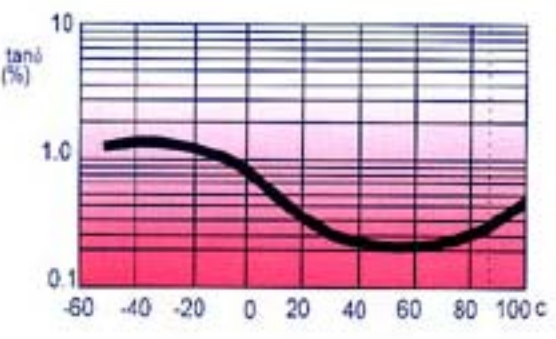
Dissipation factor (%) vs. temperature
